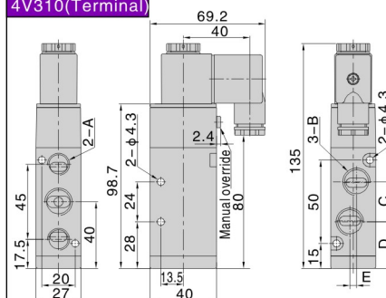
4V310(Terminal)
