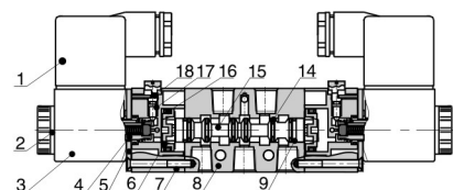
4V330C
