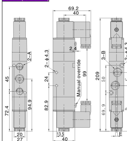
4V330(Terminal)
