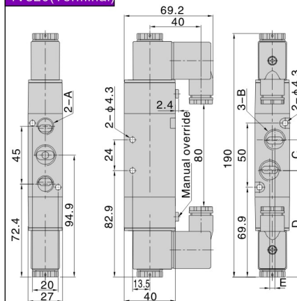
4V320(Terminal)
