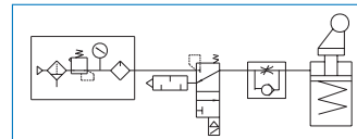
Single acting
